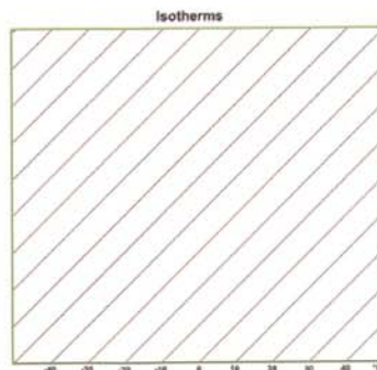
Figure 4. Isotherms, lines of equal temperature.
