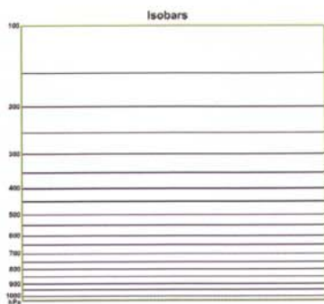
Figure 3. Isobars, lines of equal pressure. Each 100hPa represents approximately 1000m of altitude in the bottom 3000m of the atmosphere
