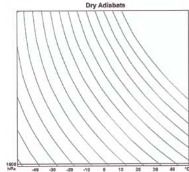
Figure 5. Dry Adiabats, the rate at which dry air cools as it ascends. When the ELR is the same as the DALR then it parallels a dry adiabat on a Skew-T
