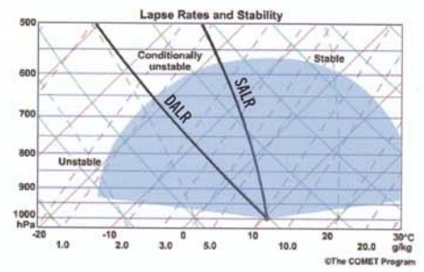
Figure 8. Different stability scenarios
